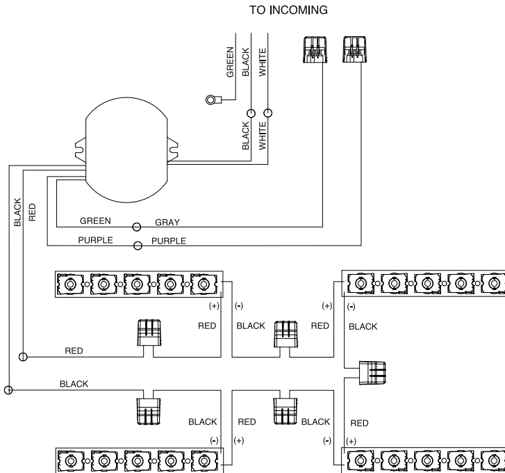
WIRING DIAGRAM
